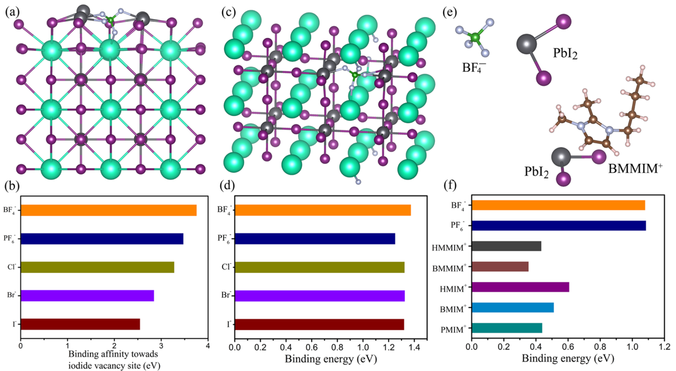
Fig. 5 a Calculated structure illustrating the passivation of an \text{I}^- vacancy at the \text{CsPbI}_2\text{Br} surface by a \text{BF}_4^- anion. b The relative interaction strengths of different anions with the \text{I}^- vacancy at the surface of the perovskite. c Calculated structure illustrating the interaction of Pb-I antisite with \text{BF}_4^- . d The binding energy of different anions with Pb-I antisite defect. e Calculated structure illustrating the interaction of \text{PbI}_2 with \text{BF}_4^- or \text{BMMIM}^+ . f The binding energy of different ions with \text{PbI}_2
