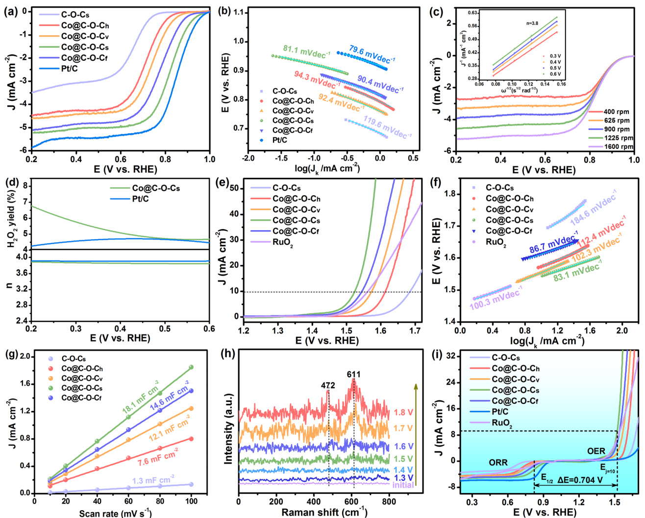
Fig. 4 a ORR LSV measurements in O_2 -saturated 1.0 \text{ mol L}^{-1} KOH solution at 1600 rpm; b Tafel plots of ORR process; c LSV curves of Co@C–O–Cs catalyst under different rotation speeds (inset: K–L plots of the Co@C–O–Cs catalyst); d Transferred electron number and H_2O_2\% of Co@C–O–Cs and Pt/C catalysts; e OER LSV measurements in O_2 -saturated 1.0 \text{ mol L}^{-1} KOH solution; f Tafel plots of OER process; g C_{dl} curves of various catalysts; h In situ Raman spectra of Co@C–O–Cs catalyst in 1.0 \text{ mol L}^{-1} KOH solution at different potentials for OER process; i Overall polarization curves of various catalysts
