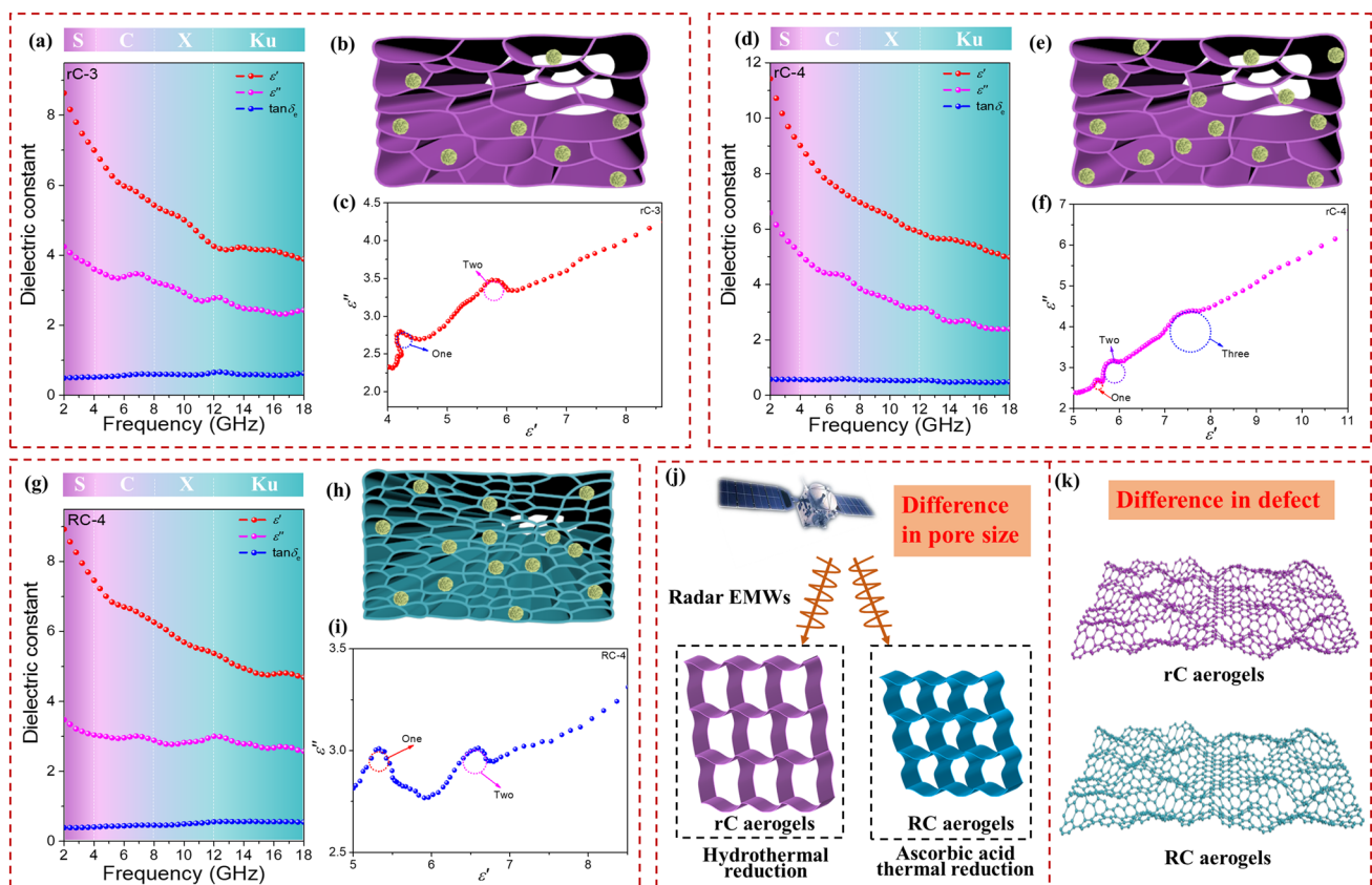
Fig. 4 \epsilon' , \epsilon'' , \tan\delta_c \sim f curves: a rC-3, d rC-4, and g RC-4. Structure diagram: b rC-3, e rC-4, and h RC-4. Cole–Cole curves: c rC-3, f rC-4, and i RC-4. Structure difference of rC and RC composite aerogels in j pore size and k number of defects
