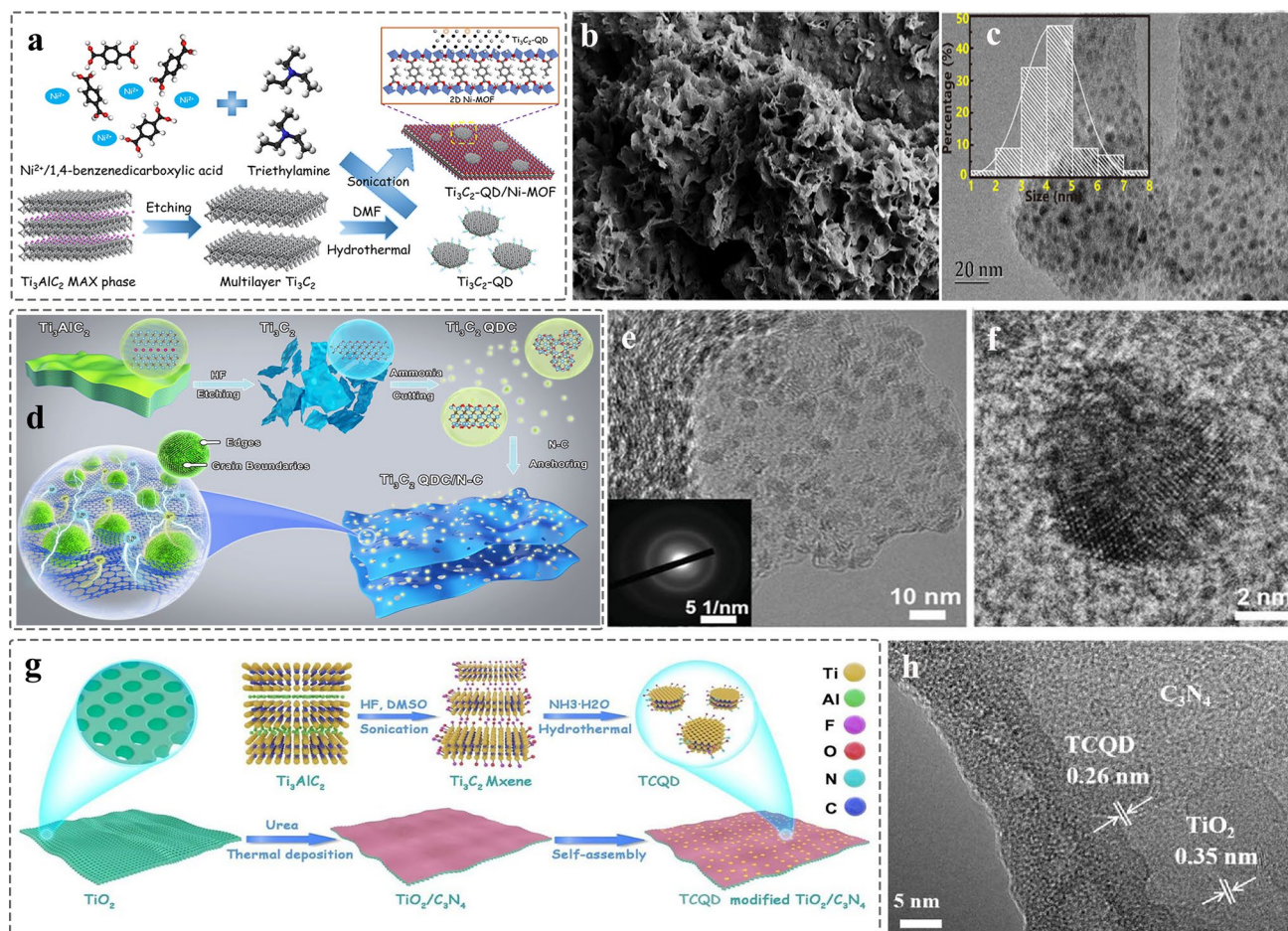
Fig. 10 Schematic and morphological and structure characterizations of 0D MQDs/2D nanosheets heterostructure. a Schematic diagram of \text{Ti}_3\text{C}_2 MQDs/Ni-MOF; b SEM images of \text{Ti}_3\text{C}_2 MQDs/Ni-MOF; c TEM images of \text{Ti}_3\text{C}_2 MQDs/Ni-MOF. The inset illustration is the size distribution of \text{Ti}_3\text{C}_2 MQDs. Reproduced with permission [69]. Copyright ©2020, American Chemical Society. d Synthesis process schematic of \text{Ti}_3\text{C}_2 QDC/N-C nanocomposites and e TEM image of \text{Ti}_3\text{C}_2 QDC/N-C, inset illustration is SAED pattern; f HRTEM image of \text{Ti}_3\text{C}_2 QDC/N-C [137]. Copyright ©2021, Wiley-VCH. g Schematic preparation of \text{Ti}_3\text{C}_2 MQDs/ \text{TiO}_2/\text{C}_3\text{N}_4 hierarchical structure; h HRTEM image of T-CN-TC heterostructure [159]. Copyright ©2020, Elsevier
