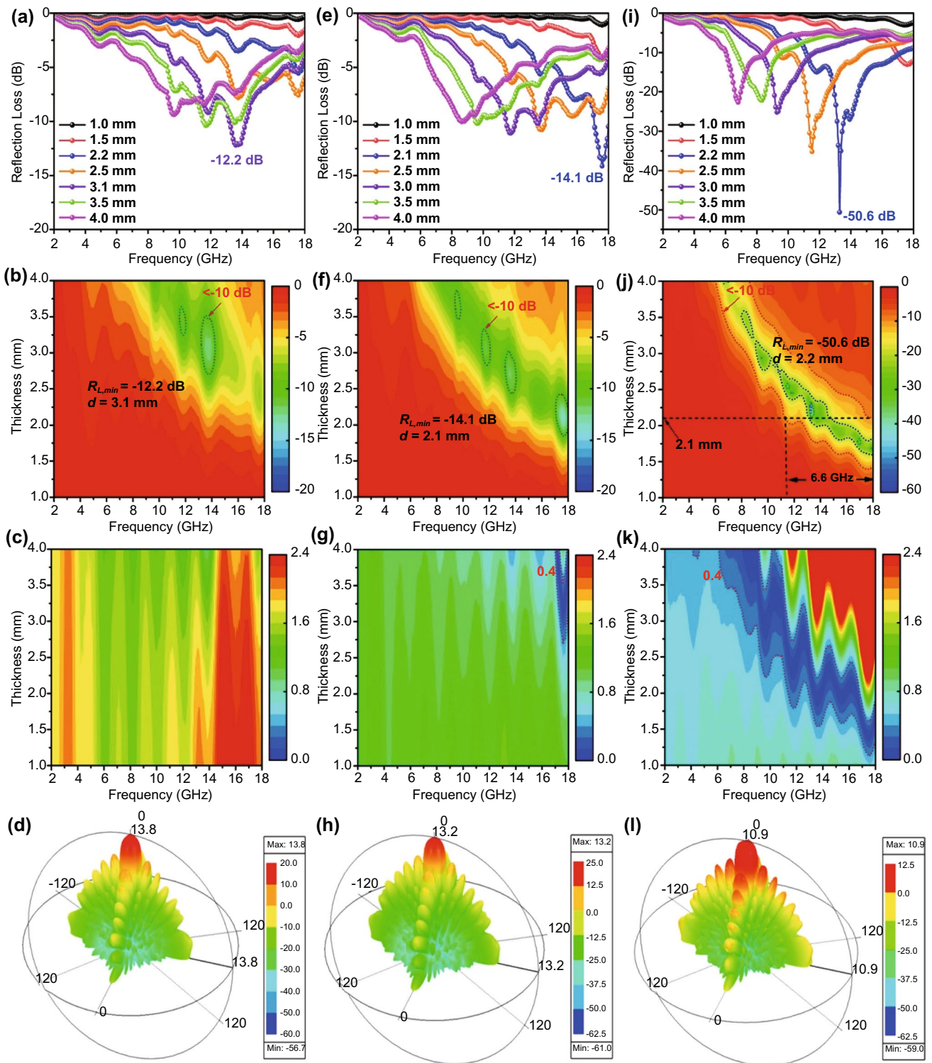
Fig. 4 R_L values, 2D projection, \Delta maps, and 3D spherical coordinate diagrams of HFSS simulation analysis for a–d \text{SiO}_2\text{@C} , e–h HCNs, and i–l \text{Co/Co}_3\text{O}_4\text{@HCNs}
